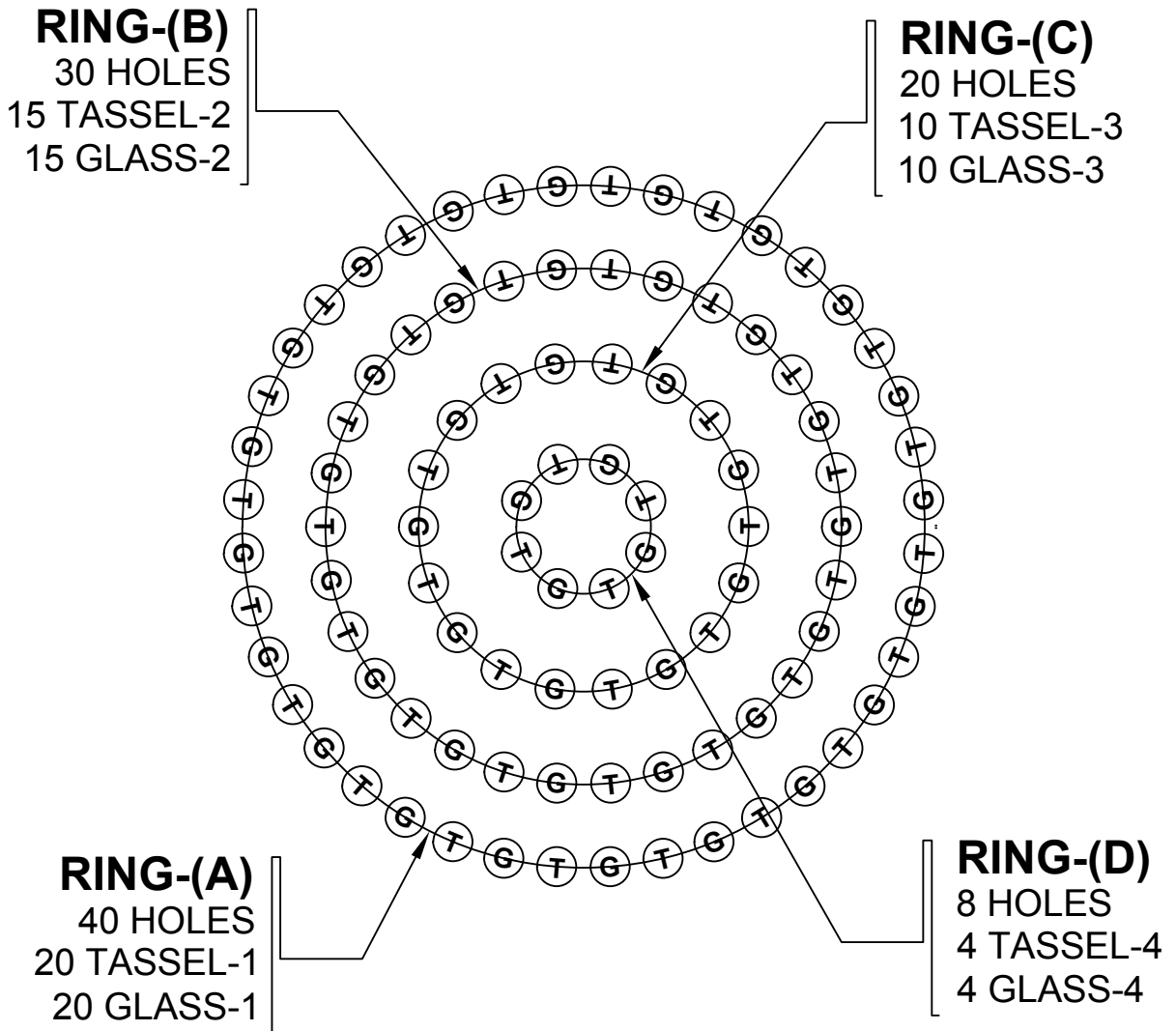
PLAN VIEW
