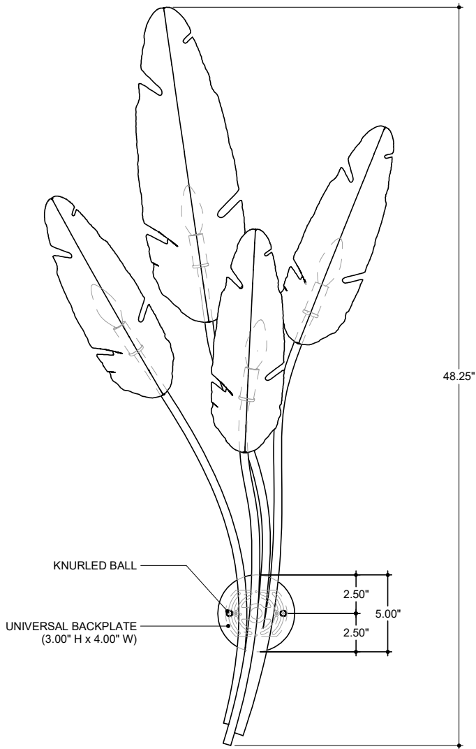
FRONT VIEW
