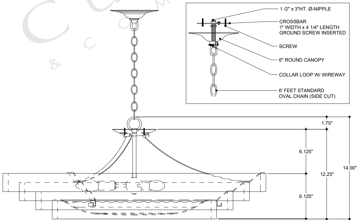
FRONT VIEW
