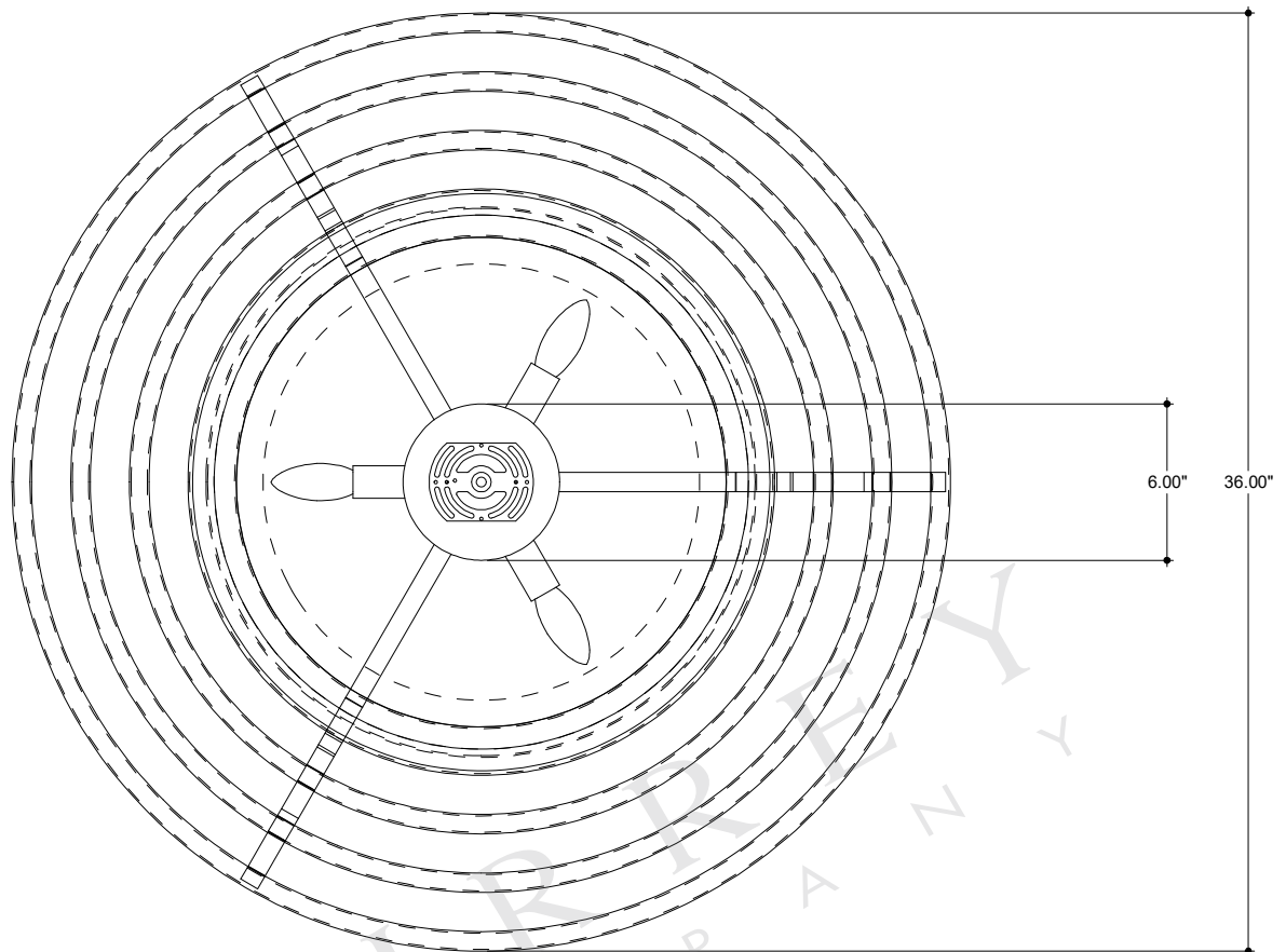
TOP VIEW
