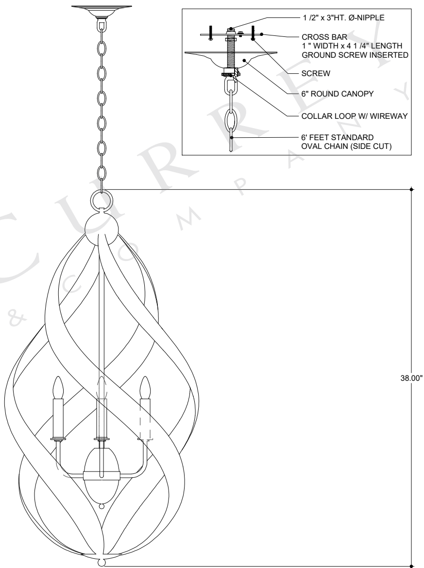
FRONT VIEW
