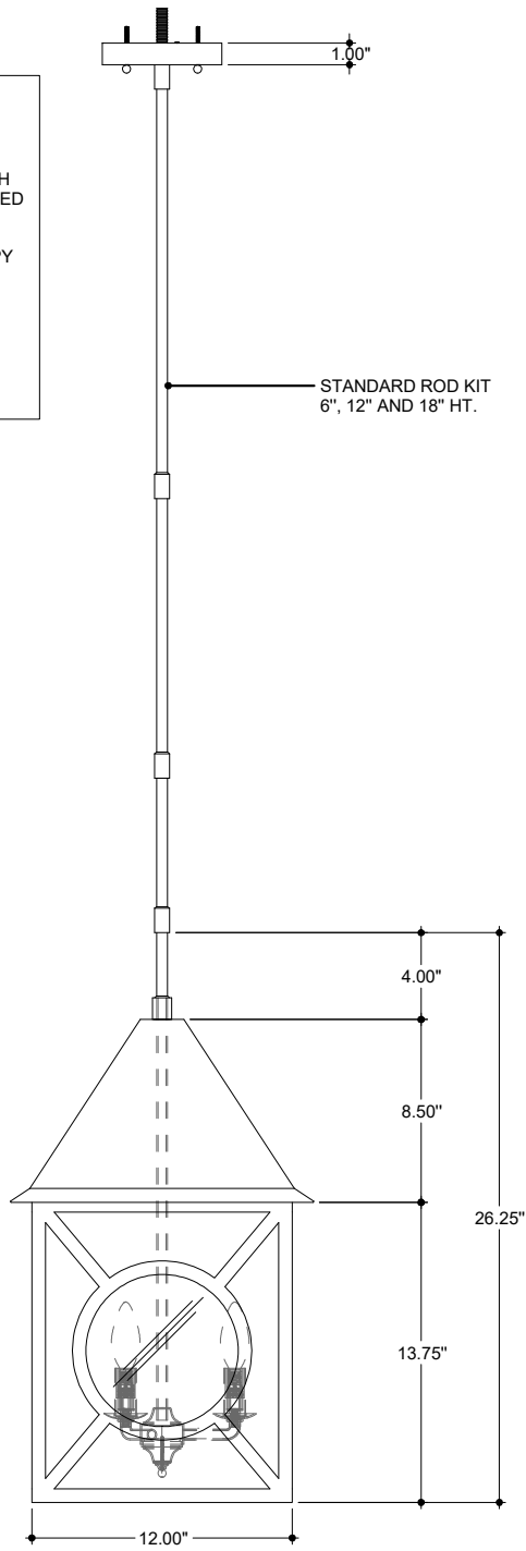
FRONT VIEW
