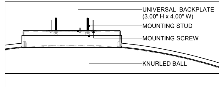
CANOPY DETAIL
