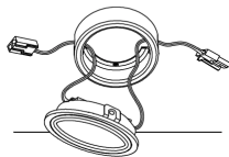
Two piece Aluminum Construction for both Surface and Recessed Installation
